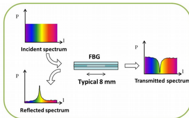
Fig.2 – Principle of FBG
